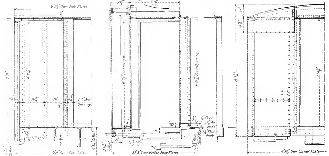
Details of Vestibule of the D. & H. Coaches
